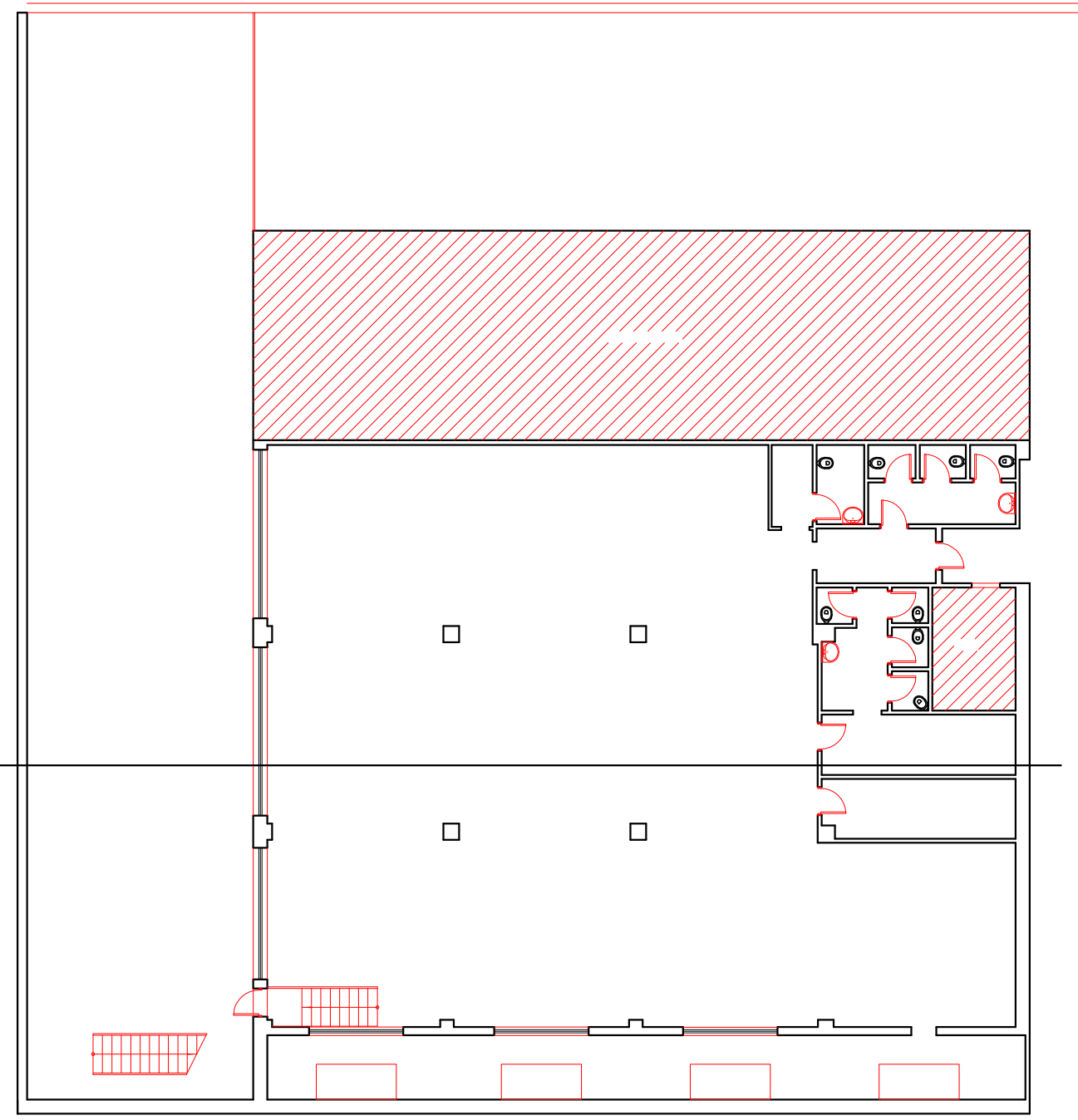
PIANO SEMINTERRATO
